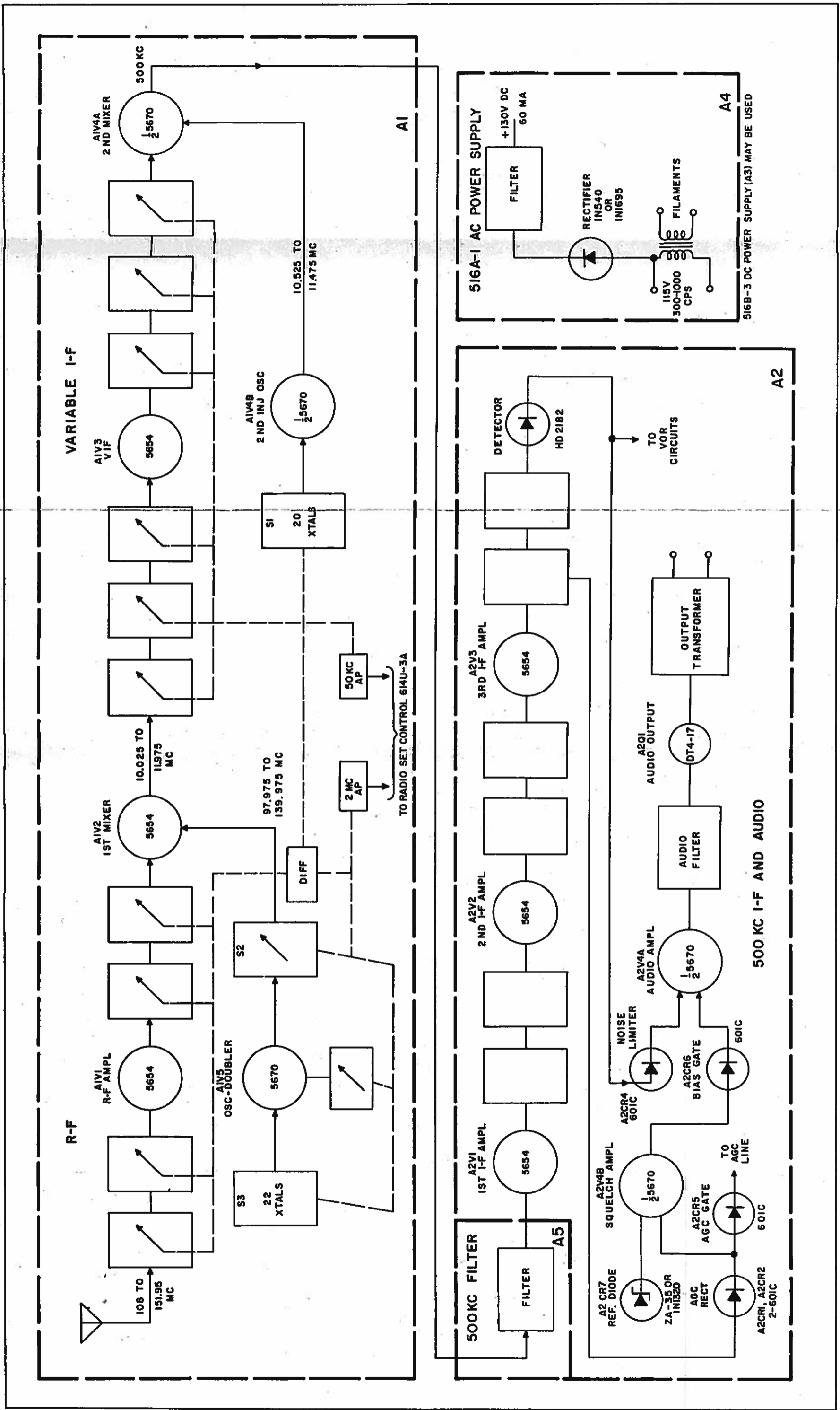
Figure 4-1. VHF Navigation and Communications Receiver 51X-2B, Block Diagram
